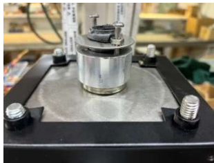
ZP-TP-LHA Top Plate Lamp Heat Sink Nut Assembly --- $147.00
